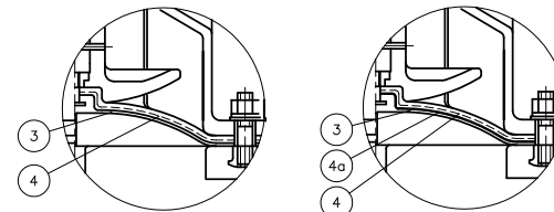
In case of PTFE Diaphragm with Cushion Cover.
